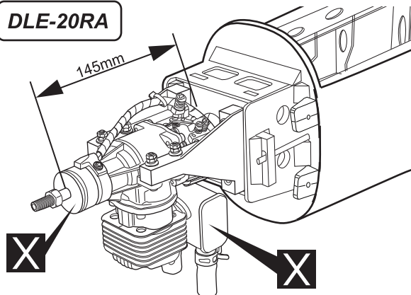
DLE 20cc with rear exhaust
